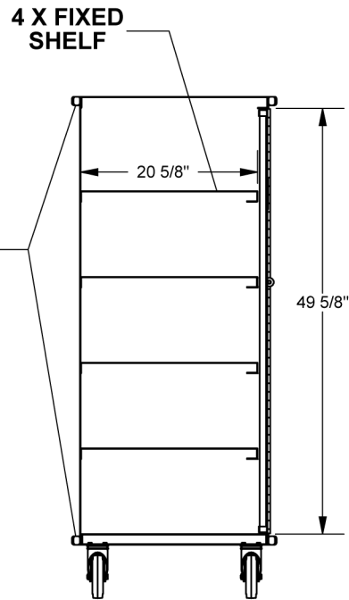
SIDE SECTION
