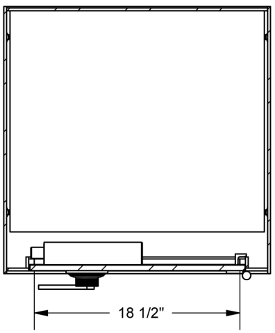
TOP SECTION
