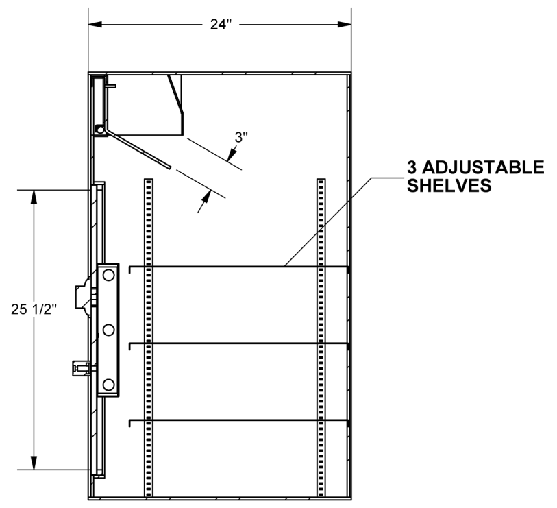
SIDE SECTION
