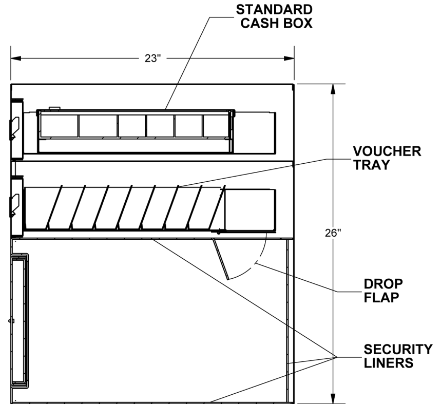
SIDE SECTION
